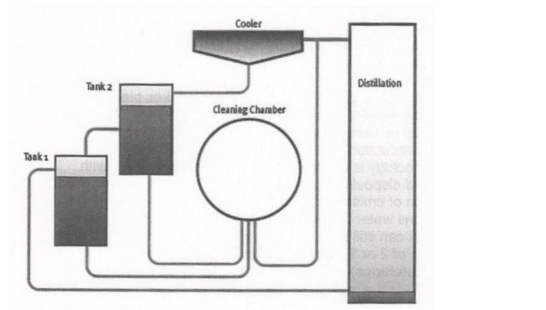
Figure 2-2 Typical cleaning equipment machine
