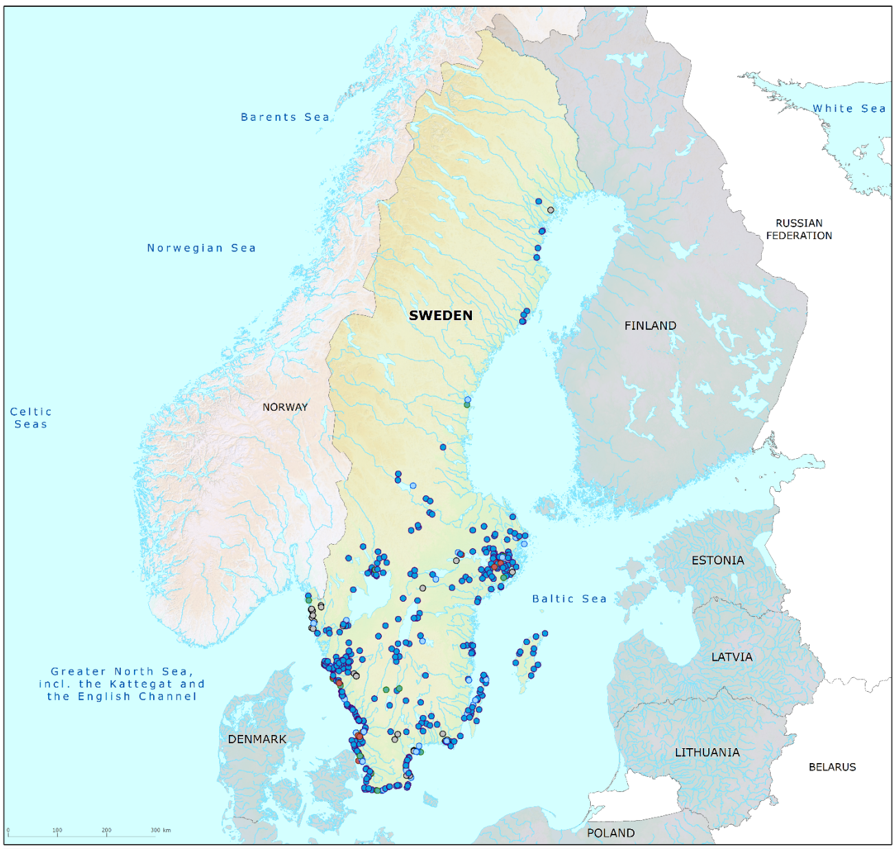
Map 1: Bathing waters reported during the 2022 bathing season in Sweden
