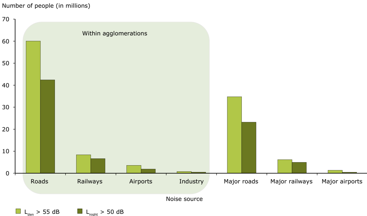
Figure 2.9 Number of people exposed to noise in Europe (EU-27, Norway and Switzerland)
