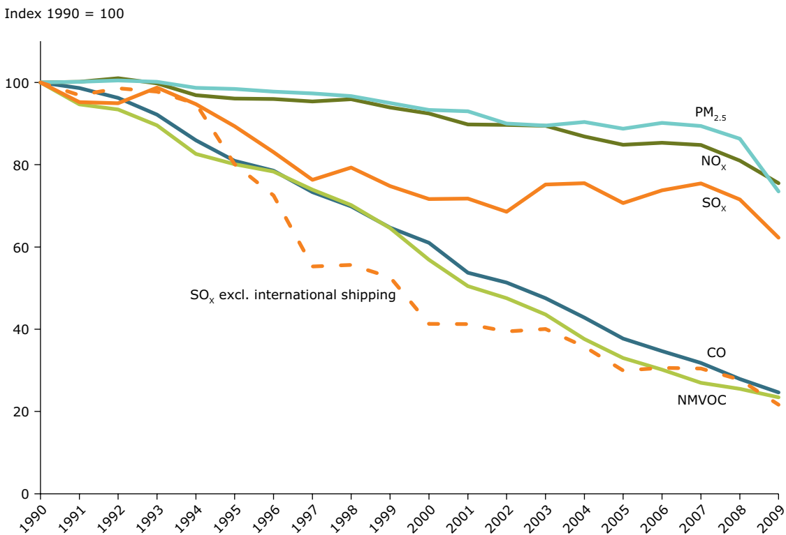
Figure 2.6 Change in emissions of main air pollutants 1990–2009 (EEA-32)
