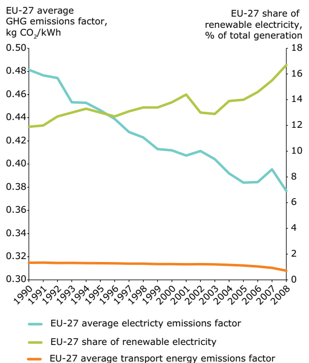
Figure 6.2 Trends in energy GHG emission factors and % renewable electricity (EU-27)
