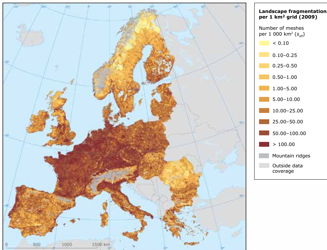
Map 2.1 Map of s_{eff} values by per 1 km 2 grid for FG-B2 in 2009
