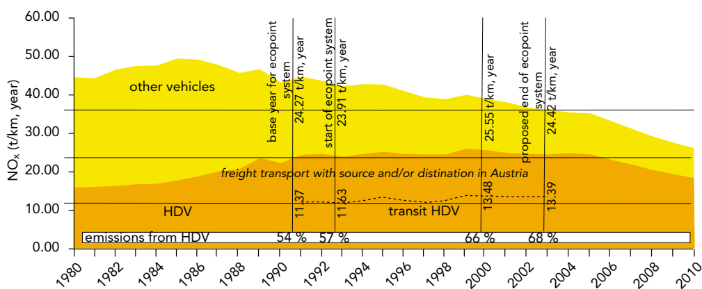
Figure A11. Changes in NO x -emissions (in t/km) on a selected section of the Brenner route (lower Inn valley, A12) at Vomp, 1980–2010
