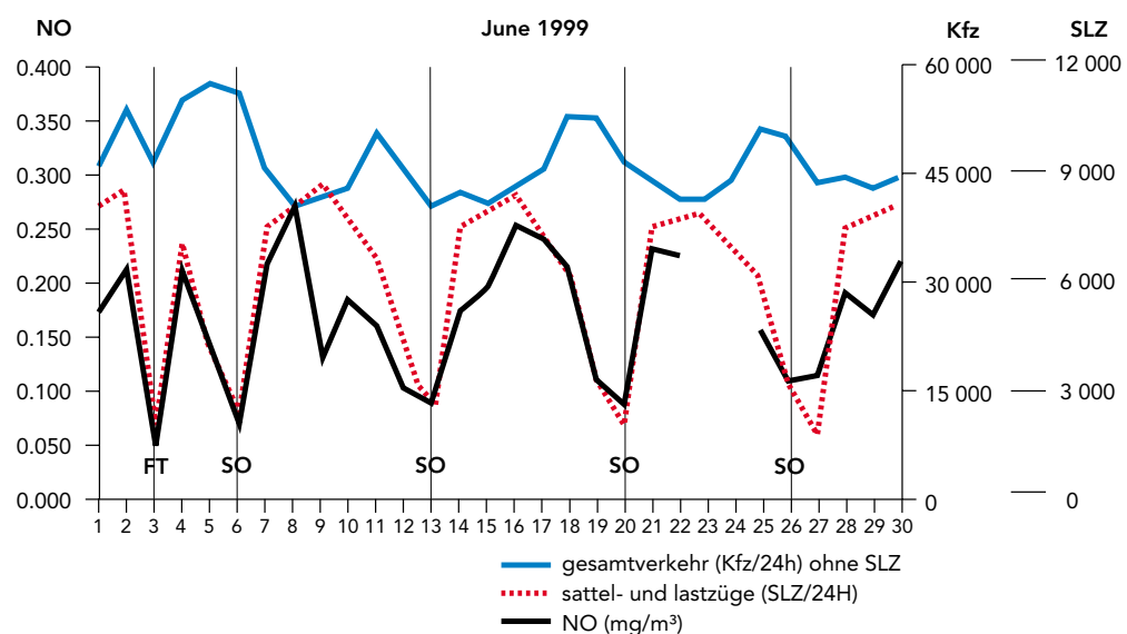
Time series of NO concentration at Vomp (A12 motorway) in June and October 1999 correlated with the traffic volumes (total vehicles and HDVs)
