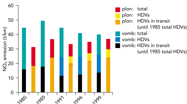
Figure A10. Estimated NO x emissions on two selected sections (A12 Vomp and A13 Plon) of the route Kufstein-Brenner
