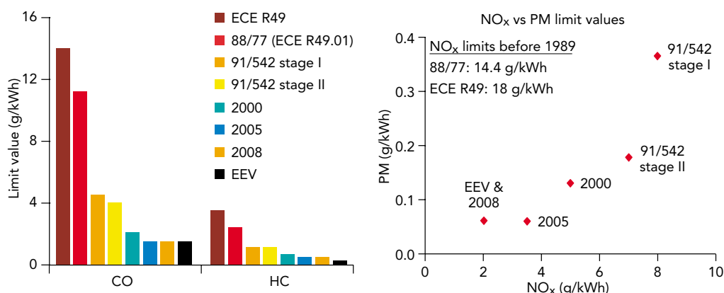
Changes in emission limits for HDVs
