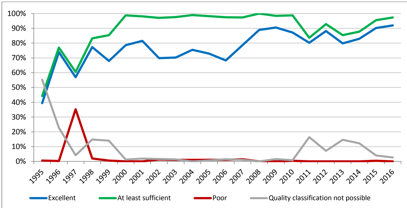
Figure 2: Inland bathing water quality trend in Finland. Note: the “At least sufficient” class also includes bathing waters of “Excellent” quality class, the sum of shares is therefore not 100%.
